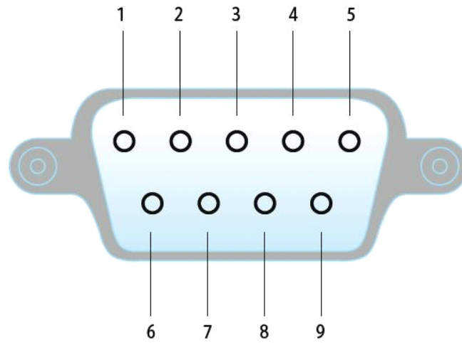
DB9 Male
